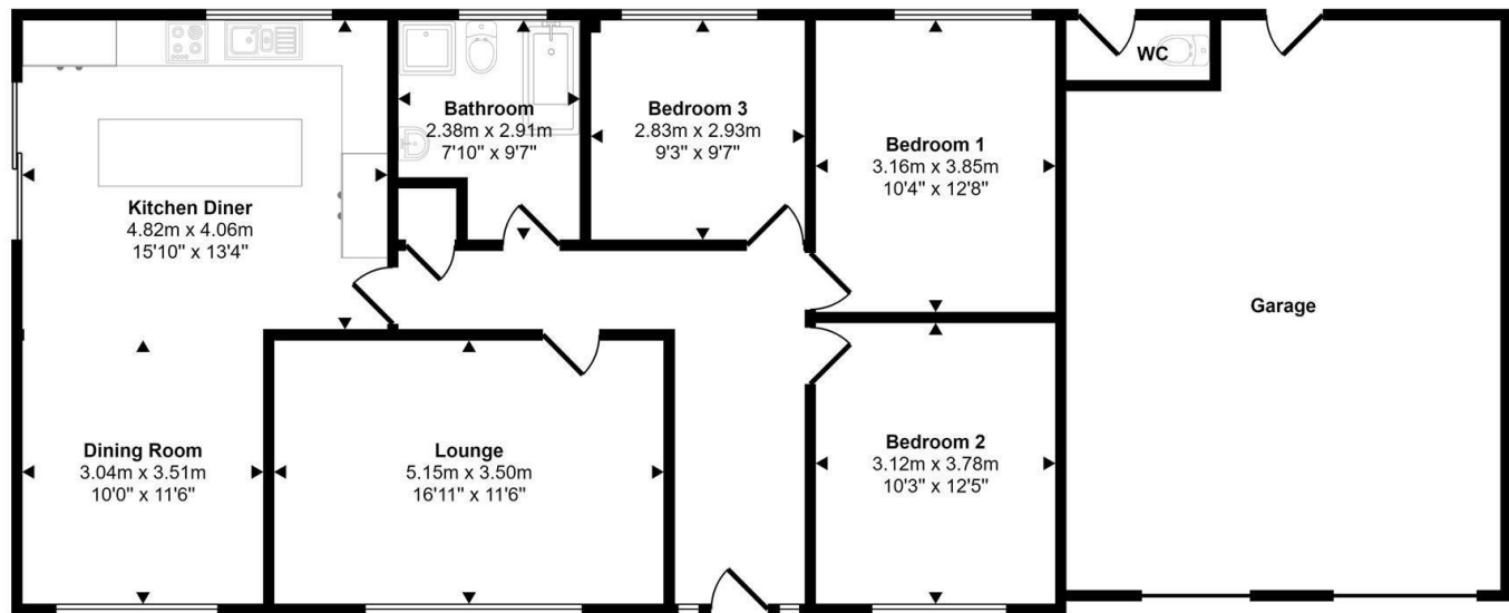
Floorplan
